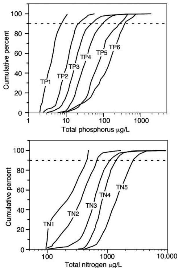
Figure 1. -Cumulative distributions of total phosphorus for each of the phosphorus zones and total nitrogen for each of the nitrogen zones. The dashed line indicates the 90th percentile that was used to find the proposed criteria for phosphorus and nitrogen.
