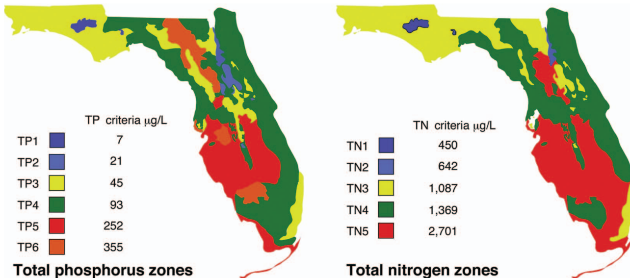
Figure 2. -Maps showing the phosphorus and nitrogen zones and the proposed numeric criteria for TP and TN.
