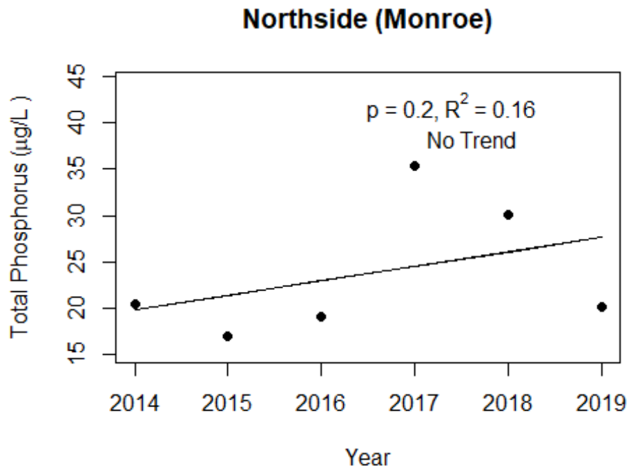
Figure 1 and Figure 2. Trend plots of annual average total phosphorus and annual average total nitrogen versus year. The R^2 value indicates the strength of the relations (ranges from 0.0 to 1.0; higher the R^2 the stronger the relation) and the p value indicates if the relation is significant ( p < 0.05 is significant). Trend Status are reported on plots.
