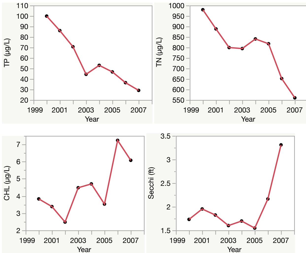
Figure 2. Lake Otter trend plots of year by average. The R^2 value indicates the strength of the relations (ranges from 0.0 to 1.0; higher the R^2 the stronger the relation) and the p value indicates if the relation is significant ( p < 0.05 is significant). Total phosphorus (TP Decreasing, R^2 = 0.89 , p = 0.00 ), total nitrogen (TN Decreasing, R^2 = 0.79 , p = 0.00 ), chlorophyll (CHL Increasing, R^2 = 0.52 , p = 0.04 ) and Secchi depth (Secchi No Trend, R^2 = 0.33 , p = 0.13 ).
