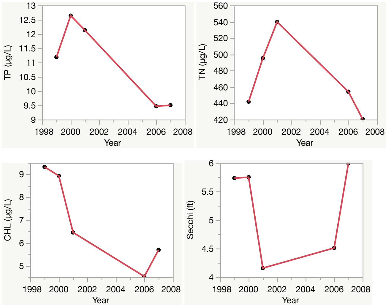
Figure 2. Lake Ellen trend plots of year by average. The R^2 value indicates the strength of the relations (ranges from 0.0 to 1.0; higher the R^2 the stronger the relation) and the p value indicates if the relation is significant ( p < 0.05 is significant). Total phosphorus (TP No Trend, R^2 = 0.75 , p = 0.06 ), total nitrogen (TN No Trend, R^2 = 0.25 , p = 0.39 ), chlorophyll (CHL Decreasing, R^2 = 0.78 , p = 0.05 ) and Secchi depth (Secchi No Trend, R^2 = 0.00 , p = 0.94 ).
