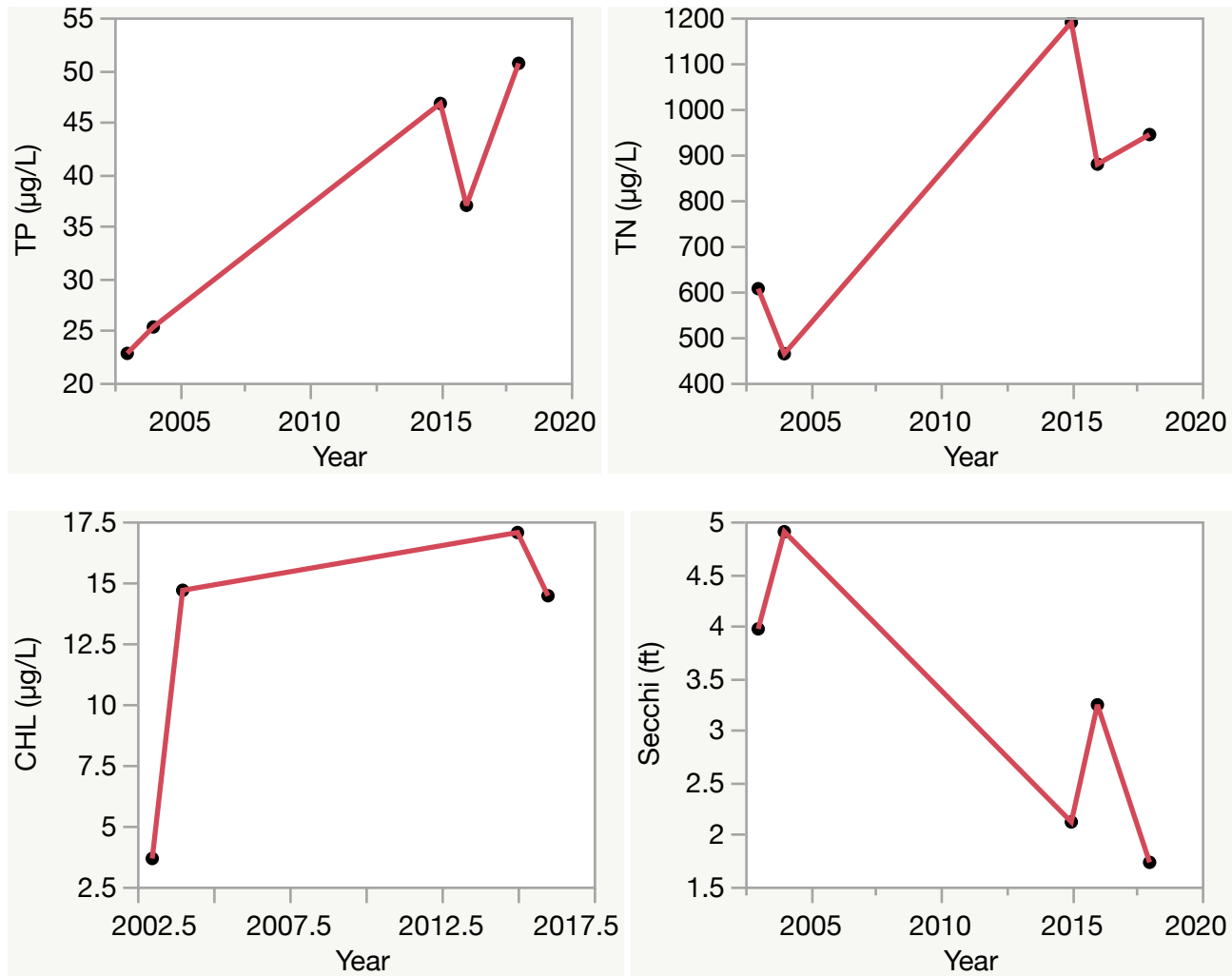
Figure 2. Lake Beluthahatchee trend plots of year by average. The R^2 value indicates the strength of the relations (ranges from 0.0 to 1.0; higher the R^2 the stronger the relation) and the p value indicates if the relation is significant ( p < 0.05 is significant). Total phosphorus (TP Increasing, R^2 = 0.87 , p = 0.02 ), total nitrogen (TN No Trend, R^2 = 0.70 , p = 0.08 ), chlorophyll (CHL No Trend, R^2 = 0.44 , p = 0.33 ) and Secchi depth (Secchi No Trend, R^2 = 0.76 , p = 0.05 ).
