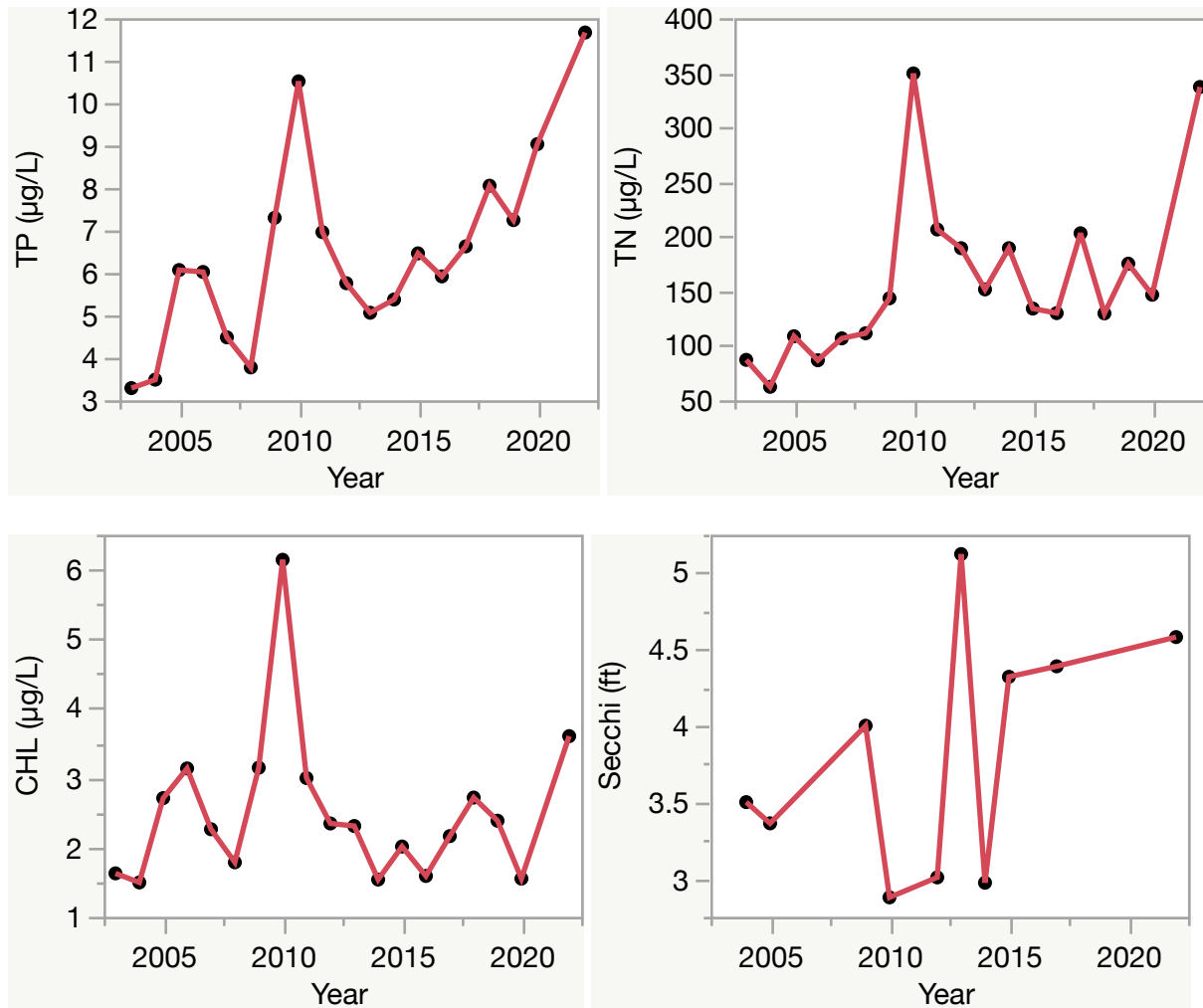
Figure 2. Lake Ski Watch trend plots of year by average. The R^2 value indicates the strength of the relations (ranges from 0.0 to 1.0; higher the R^2 the stronger the relation) and the p value indicates if the relation is significant ( p < 0.05 is significant). Total phosphorus (TP Increasing, R^2 = 0.43 , p = 0.00 ), total nitrogen (TN Increasing, R^2 = 0.26 , p = 0.03 ), chlorophyll (CHL No Trend, R^2 = 0.00 , p = 1.00 ) and Secchi depth (Secchi No Trend, R^2 = 0.24 , p = 0.15 ).
