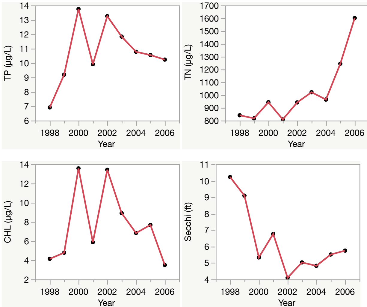
Figure 2. Lake Woodbine Springs trend plots of year by average. The R^2 value indicates the strength of the relations (ranges from 0.0 to 1.0; higher the R^2 the stronger the relation) and the p value indicates if the relation is significant ( p < 0.05 is significant). Total phosphorus (TP No Trend, R^2 = 0.09 , p = 0.44 ), total nitrogen (TN Increasing, R^2 = 0.67 , p = 0.01 ), chlorophyll (CHL No Trend, R^2 = 0.00 , p = 0.89 ) and Secchi depth (Secchi Decreasing, R^2 = 0.48 , p = 0.04 ).
