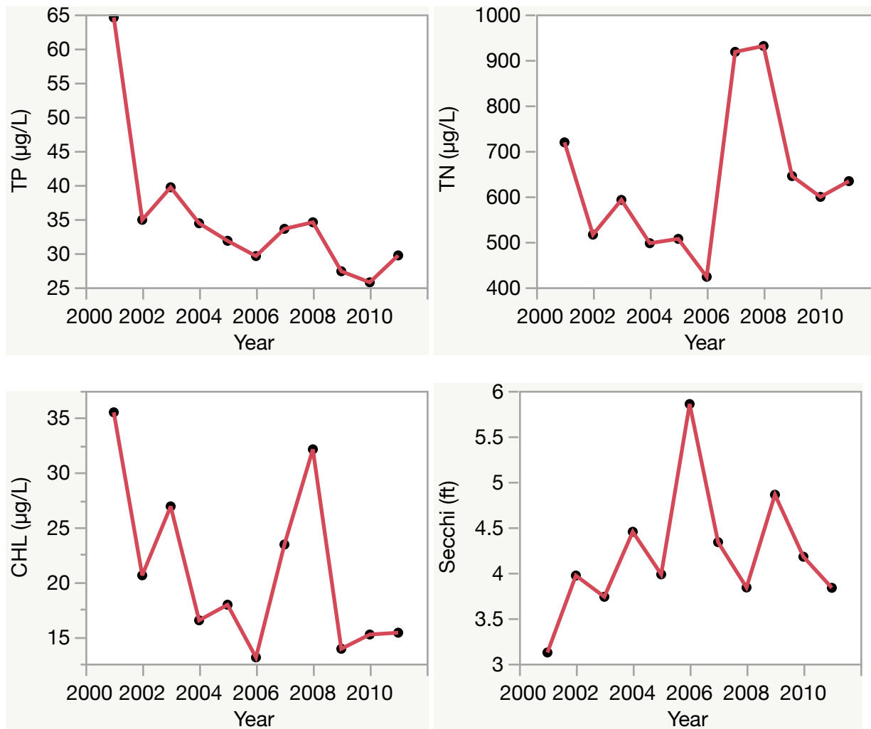
Figure 2. Lake Bear trend plots of year by average. The R^2 value indicates the strength of the relations (ranges from 0.0 to 1.0; higher the R^2 the stronger the relation) and the p value indicates if the relation is significant ( p < 0.05 is significant). Total phosphorus (TP Decreasing, R^2 = 0.50 , p = 0.02 ), total nitrogen (TN No Trend, R^2 = 0.06 , p = 0.47 ), chlorophyll (CHL No Trend, R^2 = 0.24 , p = 0.12 ) and Secchi depth (Secchi No Trend, R^2 = 0.09 , p = 0.38 ).
