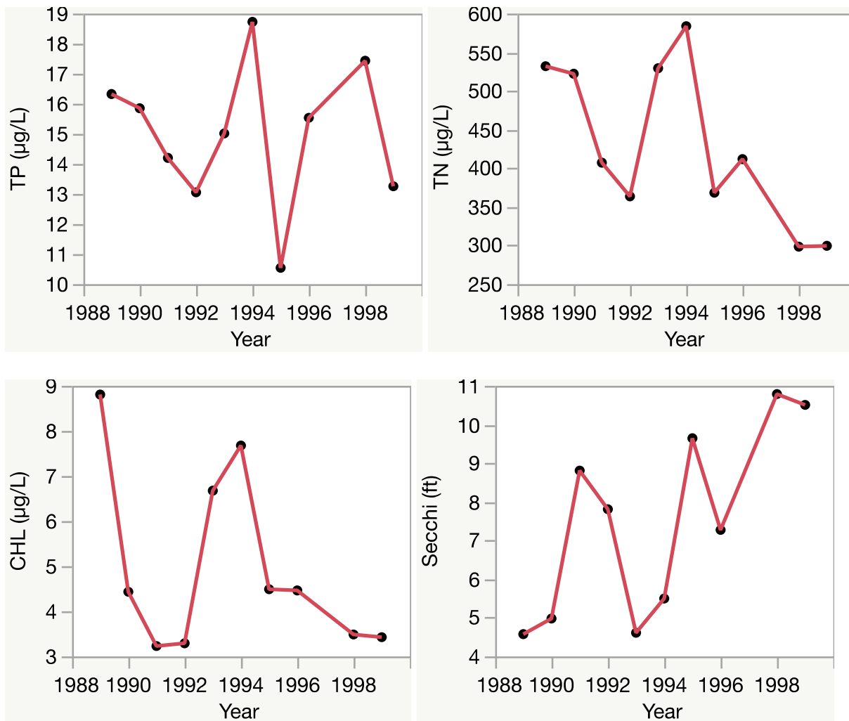
Figure 2. Lake Wooten trend plots of year by average. The R^2 value indicates the strength of the relations (ranges from 0.0 to 1.0; higher the R^2 the stronger the relation) and the p value indicates if the relation is significant ( p < 0.05 is significant). Total phosphorus (TP No Trend, R^2 = 0.01 , p = 0.81 ), total nitrogen (TN Decreasing, R^2 = 0.44 , p = 0.04 ), chlorophyll (CHL No Trend, R^2 = 0.18 , p = 0.23 ) and Secchi depth (Secchi Increasing, R^2 = 0.52 , p = 0.02 ).
