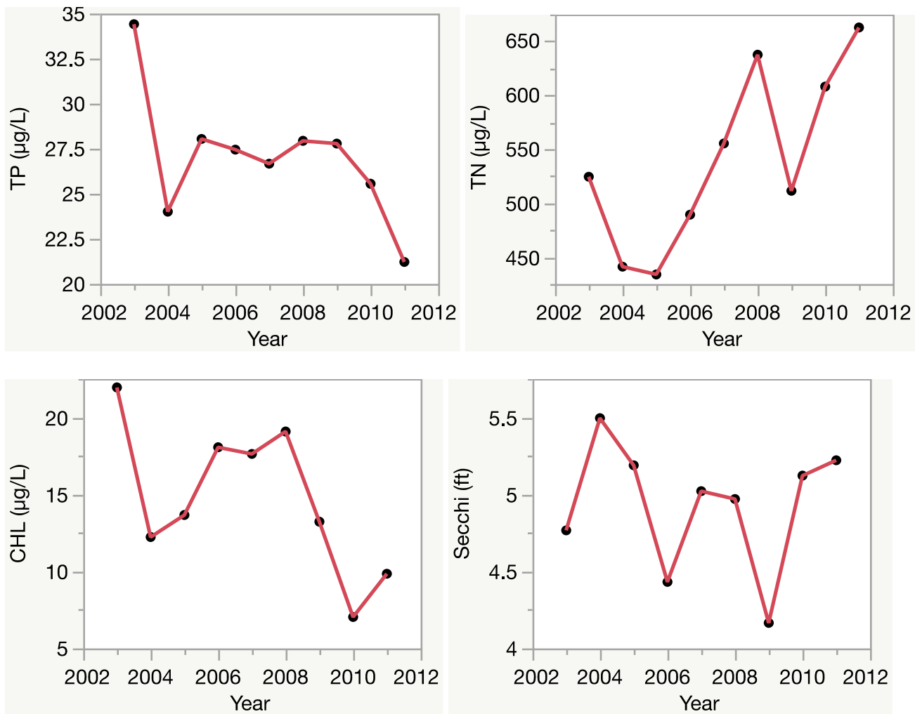
Figure 2. Lake Victor trend plots of year by average. The R^2 value indicates the strength of the relations (ranges from 0.0 to 1.0; higher the R^2 the stronger the relation) and the p value indicates if the relation is significant ( p < 0.05 is significant). Total phosphorus (TP No Trend, R^2 = 0.38 , p = 0.08 ), total nitrogen (TN Increasing, R^2 = 0.57 , p = 0.02 ), chlorophyll (CHL No Trend, R^2 = 0.37 , p = 0.08 ) and Secchi depth (Secchi No Trend, R^2 = 0.01 , p = 0.82 ).
