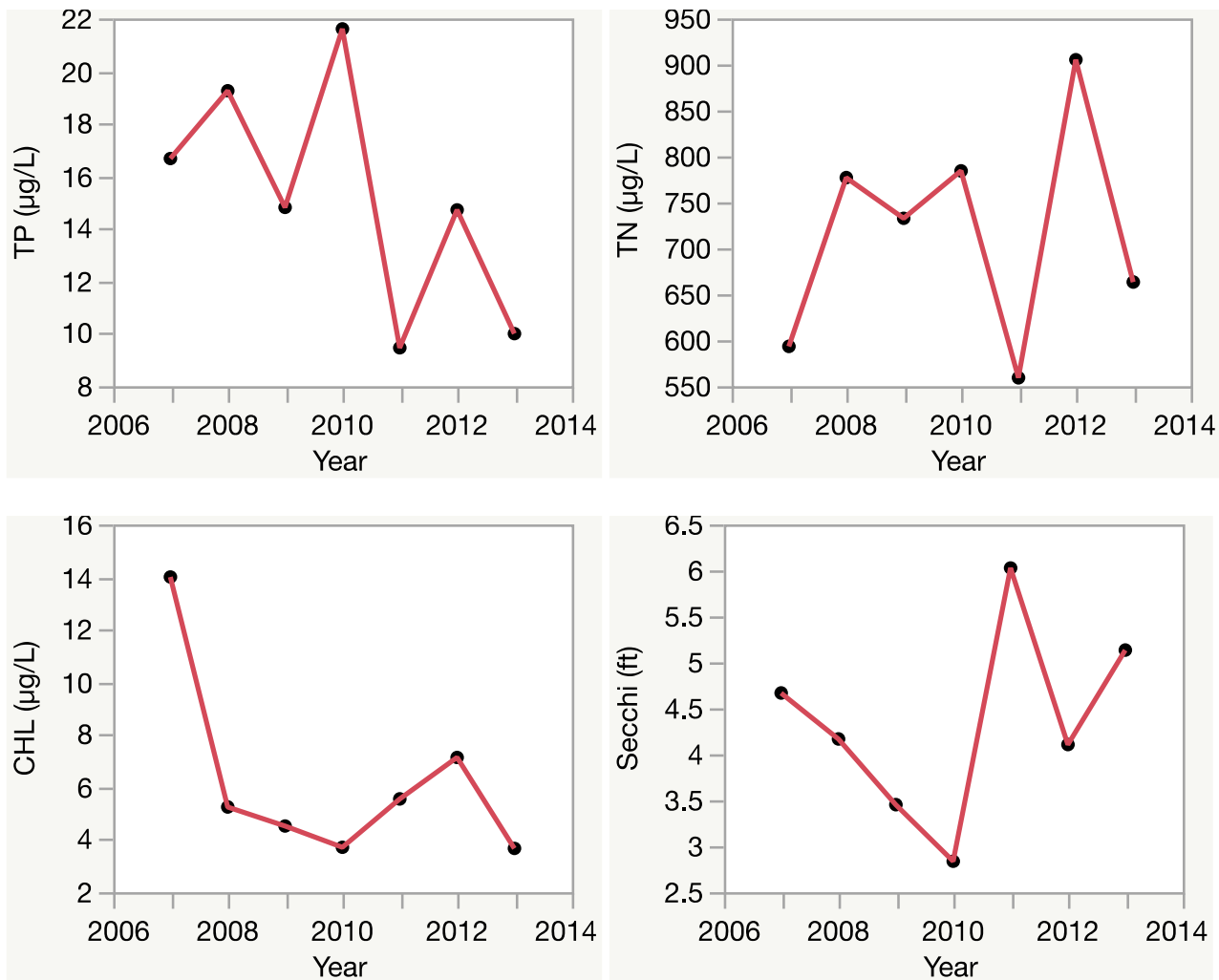
Figure 2. Lake Dead trend plots of year by average. The R^2 value indicates the strength of the relations (ranges from 0.0 to 1.0; higher the R^2 the stronger the relation) and the p value indicates if the relation is significant ( p < 0.05 is significant). Total phosphorus (TP No Trend, R^2 = 0.35 , p = 0.16 ), total nitrogen (TN No Trend, R^2 = 0.04 , p = 0.69 ), chlorophyll (CHL No Trend, R^2 = 0.31 , p = 0.19 ) and Secchi depth (Secchi No Trend, R^2 = 0.08 , p = 0.54 ).
