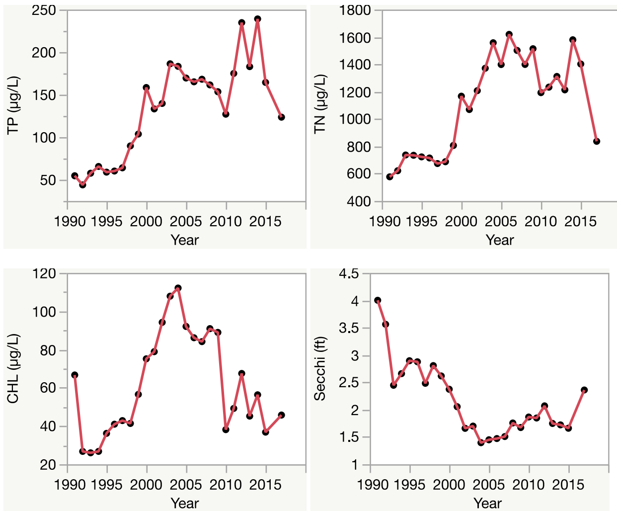
Figure 2. Lake Tallavana trend plots of year by average. The R^2 value indicates the strength of the relations (ranges from 0.0 to 1.0; higher the R^2 the stronger the relation) and the p value indicates if the relation is significant ( p < 0.05 is significant). Total phosphorus (TP Increasing, R^2 = 0.65 , p = 0.00 ), total nitrogen (TN Increasing, R^2 = 0.50 , p = 0.00 ), chlorophyll (CHL No Trend, R^2 = 0.05 , p = 0.29 ) and Secchi depth (Secchi Decreasing, R^2 = 0.51 , p = 0.00 ).
