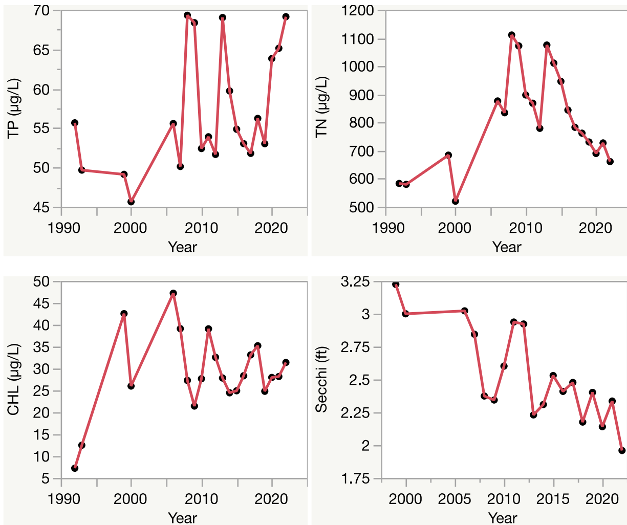
Figure 2. Lake Talquin trend plots of year by average. The R^2 value indicates the strength of the relations (ranges from 0.0 to 1.0; higher the R^2 the stronger the relation) and the p value indicates if the relation is significant ( p < 0.05 is significant). Total phosphorus (TP Increasing, R^2 = 0.19 , p = 0.05 ), total nitrogen (TN No Trend, R^2 = 0.08 , p = 0.21 ), chlorophyll (CHL No Trend, R^2 = 0.09 , p = 0.18 ) and Secchi depth (Secchi Decreasing, R^2 = 0.65 , p = 0.00 ).
