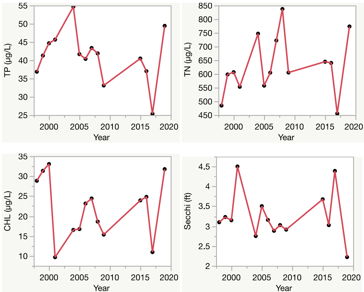
Figure 2. Lake Yvette trend plots of year by average. The R^2 value indicates the strength of the relations (ranges from 0.0 to 1.0; higher the R^2 the stronger the relation) and the p value indicates if the relation is significant ( p < 0.05 is significant). Total phosphorus (TP No Trend, R^2 = 0.07 , p = 0.35 ), total nitrogen (TN No Trend, R^2 = 0.06 , p = 0.41 ), chlorophyll (CHL No Trend, R^2 = 0.01 , p = 0.68 ) and Secchi depth (Secchi No Trend, R^2 = 0.01 , p = 0.77 ).
