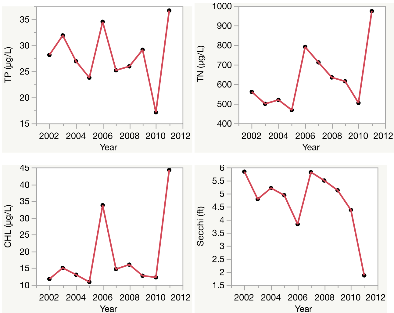
Figure 2. Lake Stone trend plots of year by average. The R^2 value indicates the strength of the relations (ranges from 0.0 to 1.0; higher the R^2 the stronger the relation) and the p value indicates if the relation is significant ( p < 0.05 is significant). Total phosphorus (TP No Trend, R^2 = 0.00 , p = 0.87 ), total nitrogen (TN No Trend, R^2 = 0.29 , p = 0.11 ), chlorophyll (CHL No Trend, R^2 = 0.19 , p = 0.21 ) and Secchi depth (Secchi No Trend, R^2 = 0.30 , p = 0.10 ).
