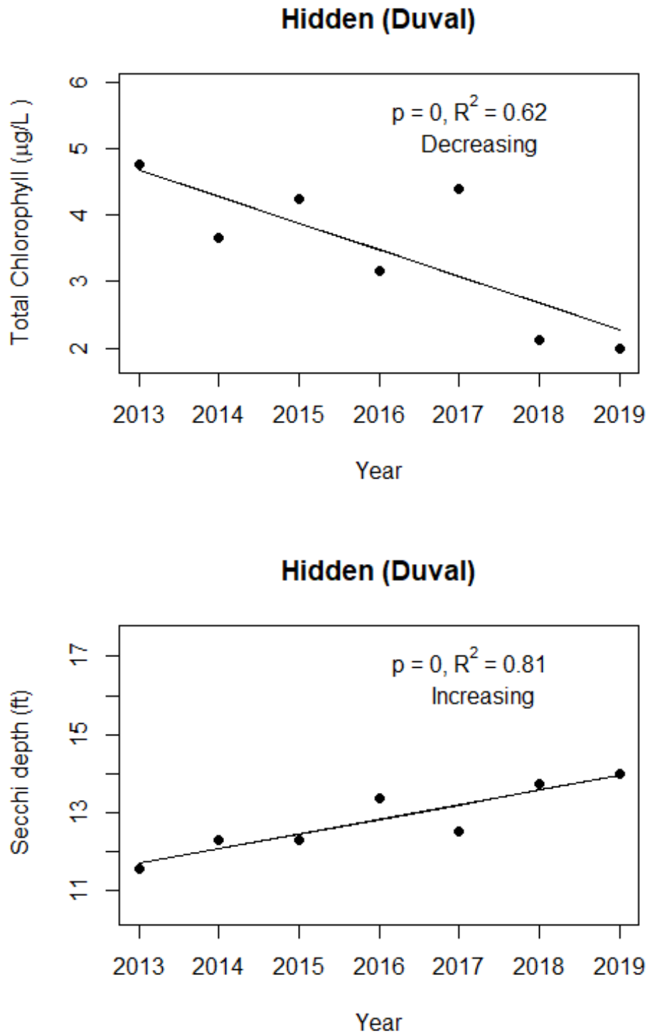
Figure 3 and Figure 4. Trend plots of annual average chlorophyll and annual average Secchi versus year. The R2 value indicates the strength of the relations (ranges from 0.0 to 1.0; higher the R2 the stronger the relations and the p value indicates if the relation is significant (p < 0.05 is significant). Trend status are reported on plots.
