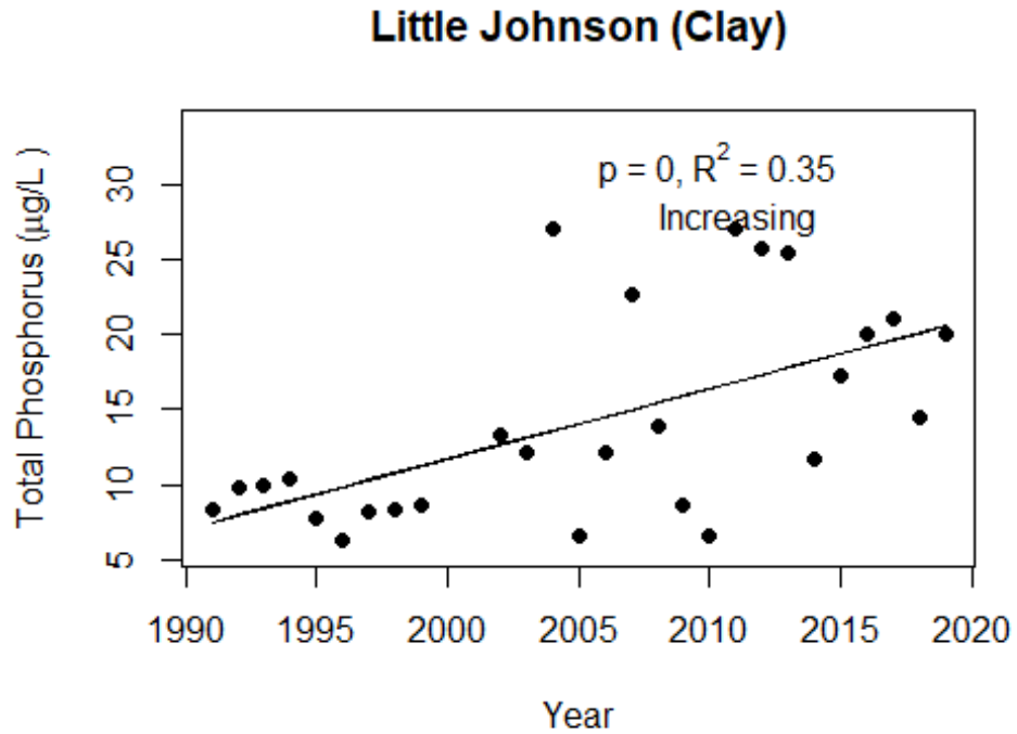
Figure 1 and Figure 2. Trend plots of annual average total phosphorus and annual average total nitrogen versus year. The R^2 value indicates the strength of the relations (ranges from 0.0 to 1.0; higher the R^2 the stronger the relation) and the p value indicates if the relation is significant ( p < 0.05 is significant). Trend Status are reported on plots.
