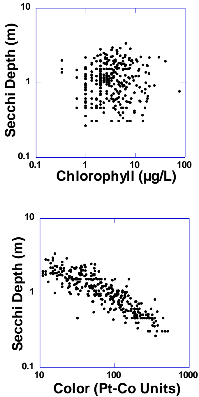
Figure 8. Relations between Secchi depth and chlorophyll (Top), and Secchi depth and color (Bottom) for the Walton County dune lakes using Florida LAKEWATCH data.
