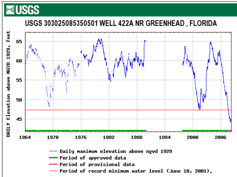
Figure 3. Long-term record for water table elevation in a well monitored by USGS and located in Greenhead, Florida approximately 25 miles northeast of the Walton County Dune lakes.
