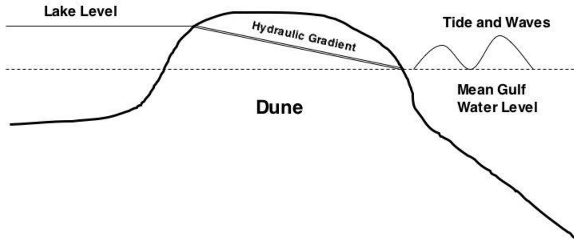
Figure 6. Schematic of water table elevation across a sand dune between a coastal lake and a tidally influenced Gulf of Mexico.
