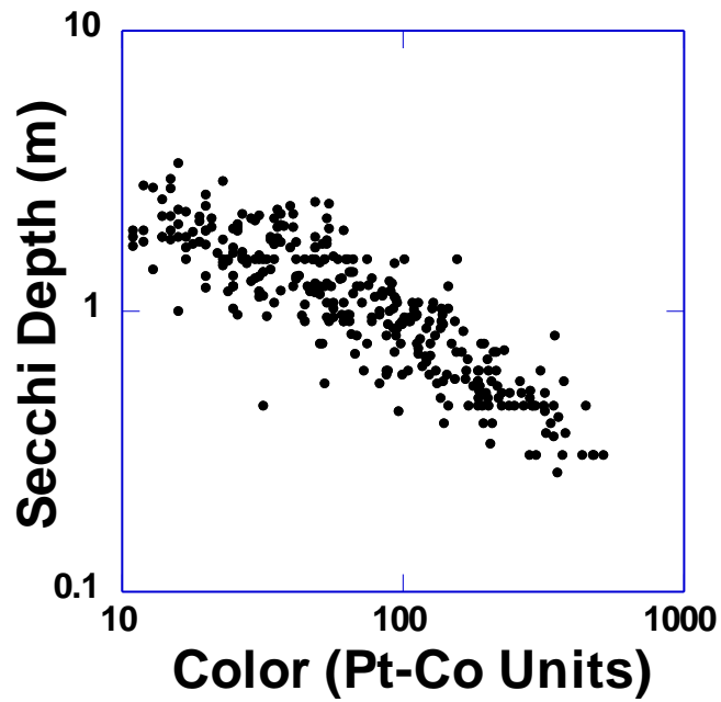
Figure 8. Relations between Secchi depth and chlorophyll (Top), and Secchi depth and color (Bottom) for the Walton County dune lakes using Florida LAKEWATCH data.
