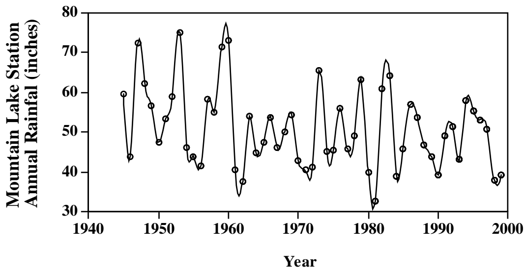
Figure 2. Lake level deviation from long-term average lake level for 36 lakes on the Lake Wales Ridge including Lake Wailes and long-term rainfall records.
