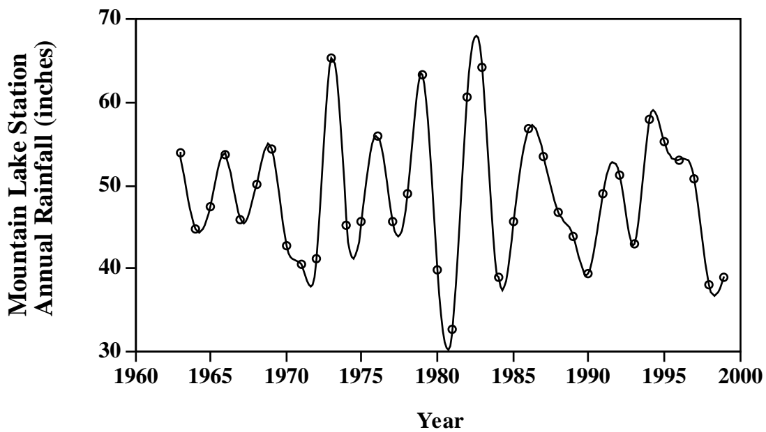
Figure 1. Long-term monthly water level (ft MSL) and long-term rainfall (inches) for Lake Wailes.
